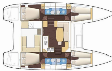
Plan version 4 cabins 4 SBD* / 4 cabins version - 4 washrooms
